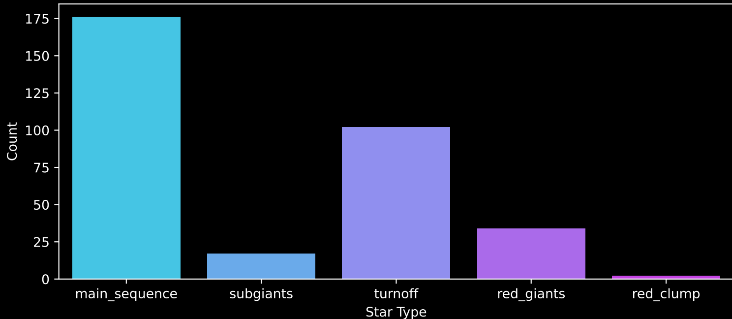
GALAH DR4 Field: [217] Count plot of Star Type
