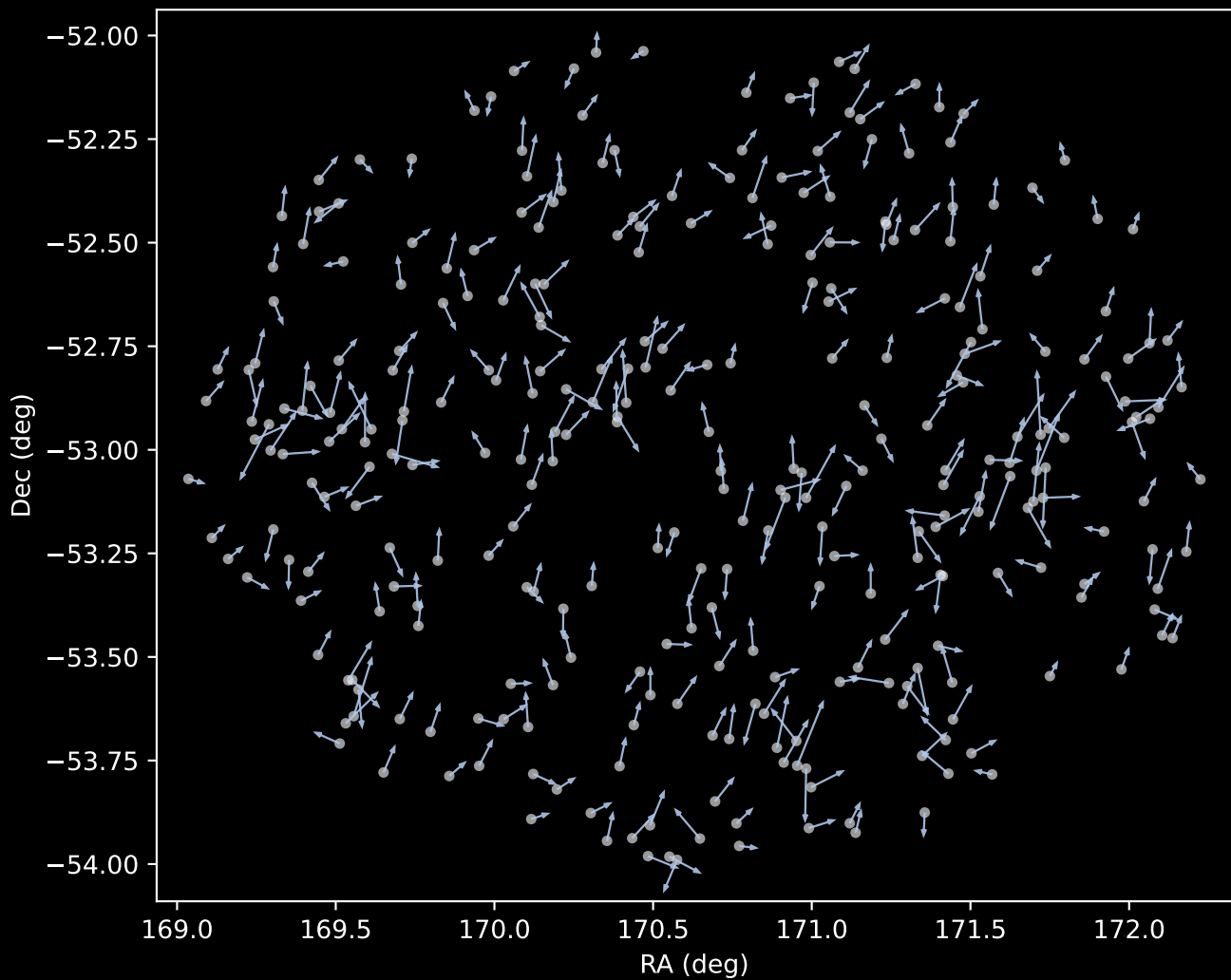
GALAH DR4 Cluster 1 Proper Motion Vectors (n=308)
