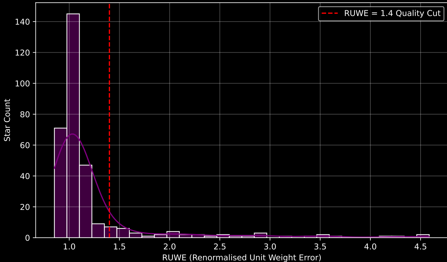
GALAH DR4 Field [217] RUWE Distribution (n= 316)
