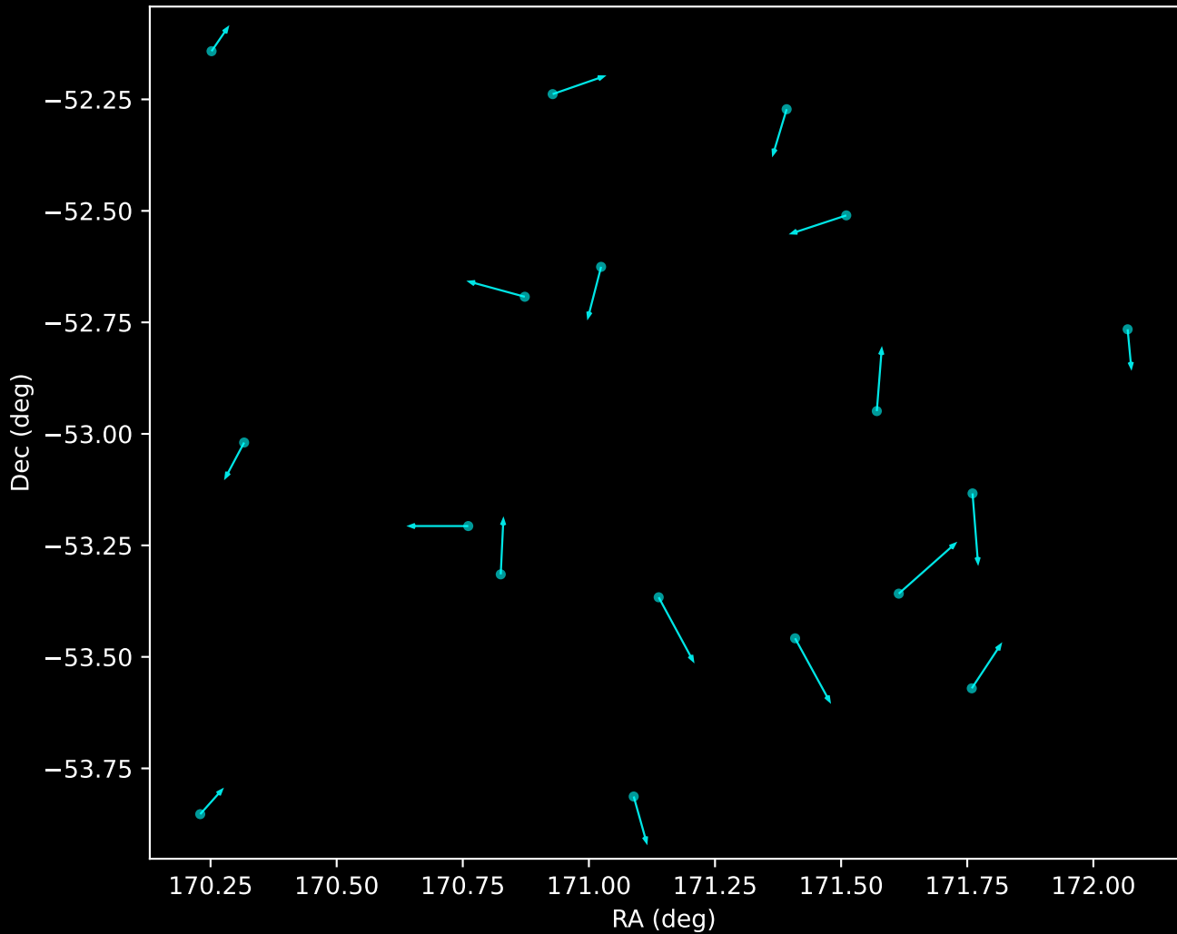
GALAH DR4 Noise Stream Proper Motion Vectors (n=18)
